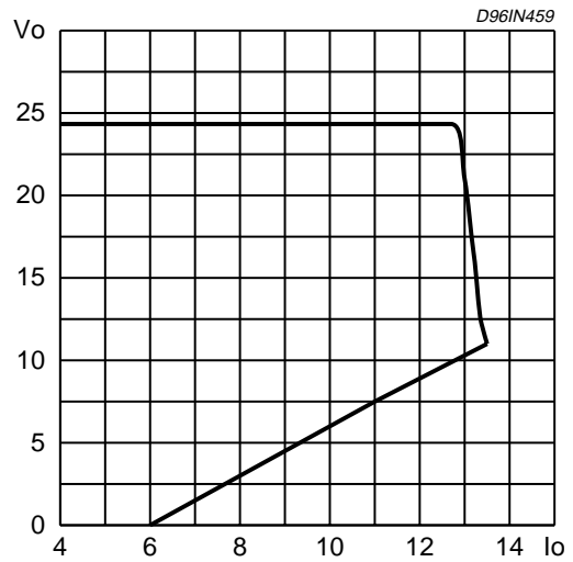
Figure 4b: Output limiting current characteristic
