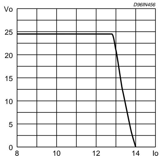
Figure 2: Output limiting current characteristic using two current transformers
